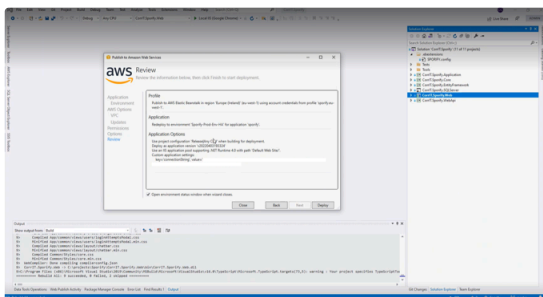
Review Modal
