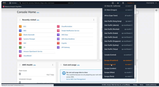
Region Select
