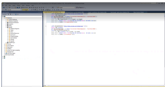
Execute script
