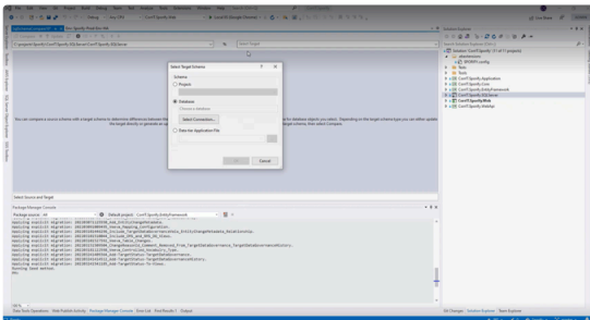
Schema Compare
